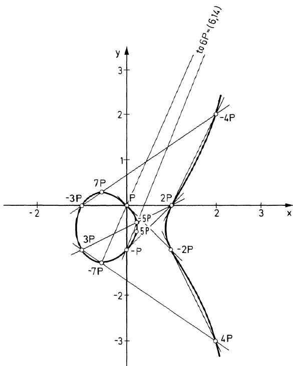
Fig. 1. The curve y^2 + y = x^3 - x
